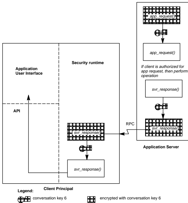
Figure 24–9. Application Server Responds to Client's Request
