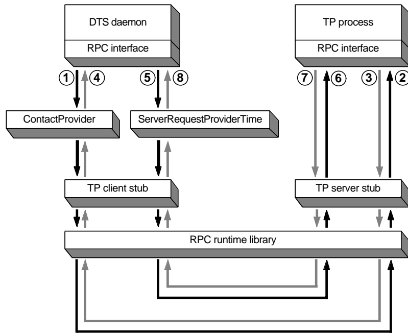
Figure 21–1. DTS/Time-Provider RPC Calling Sequence
