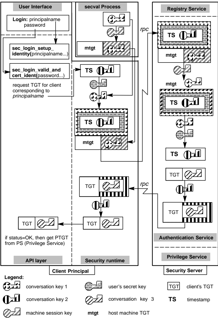
Figure 24–4. Client Acquires TGT Using Third-Party Protocol
