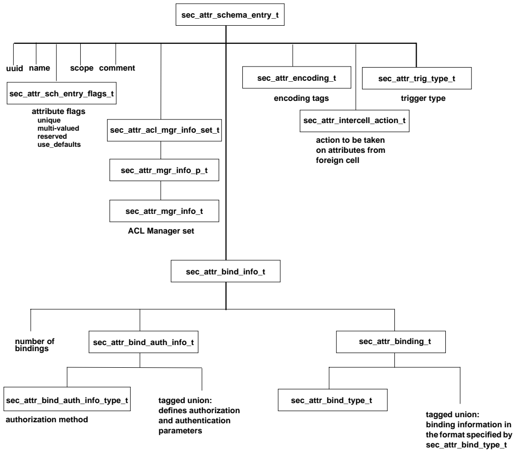
Figure 29–1. The sec_attr_schema_entry_t Data Type
