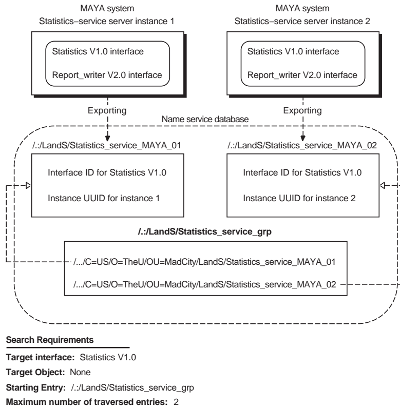
Figure 14–16. Service Model: Distinct Instances on One Host
