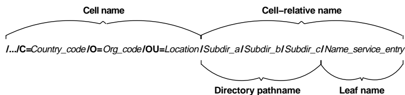
Figure 14–8. Parts of a Global Name
