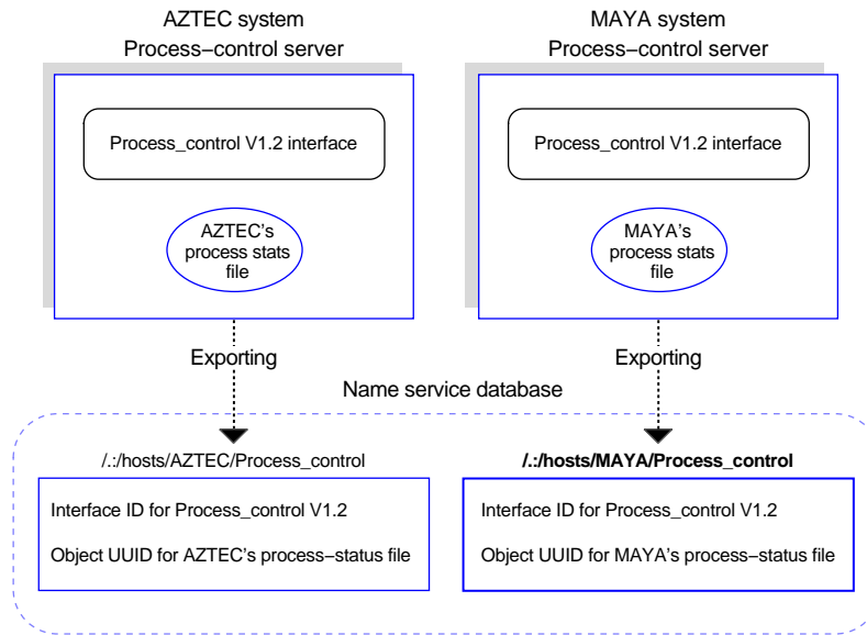
Figure 14–17. Resource Model: A System-Specific Application
