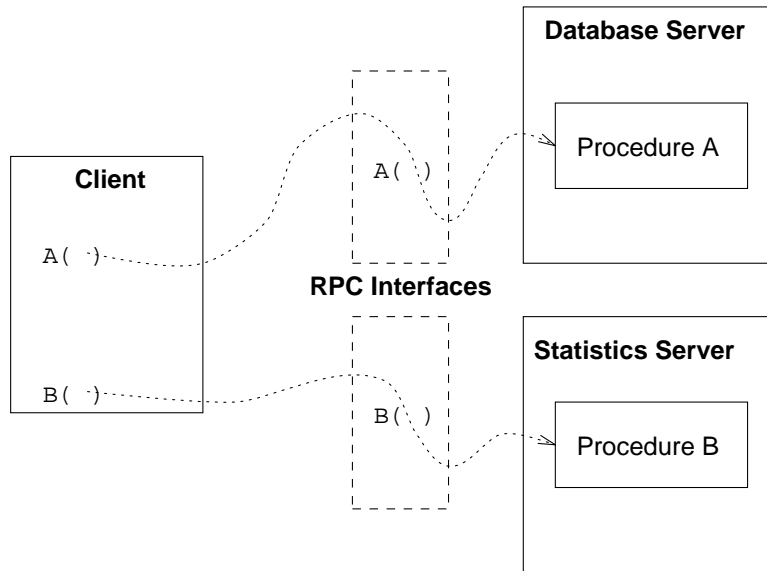
Figure 11–6. Role of RPC Interfaces
