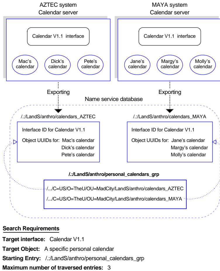
Figure 14–18. Resource Model: A Single Server Entry for Each Server
