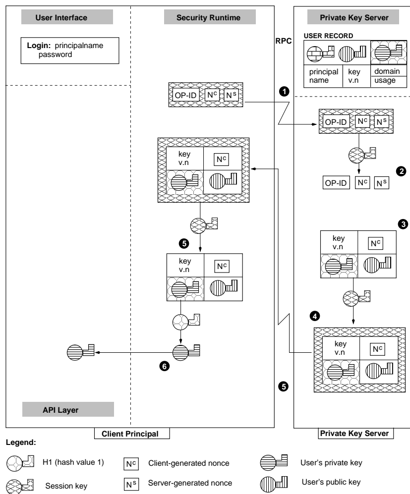
Figure 24–3. Client Acquisition of Private Key from PKSS
