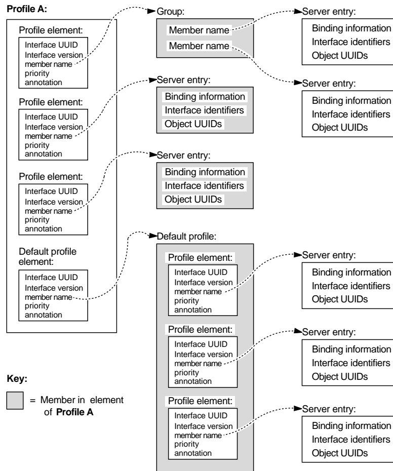
Figure 14–11. Possible Mappings of a Profile
