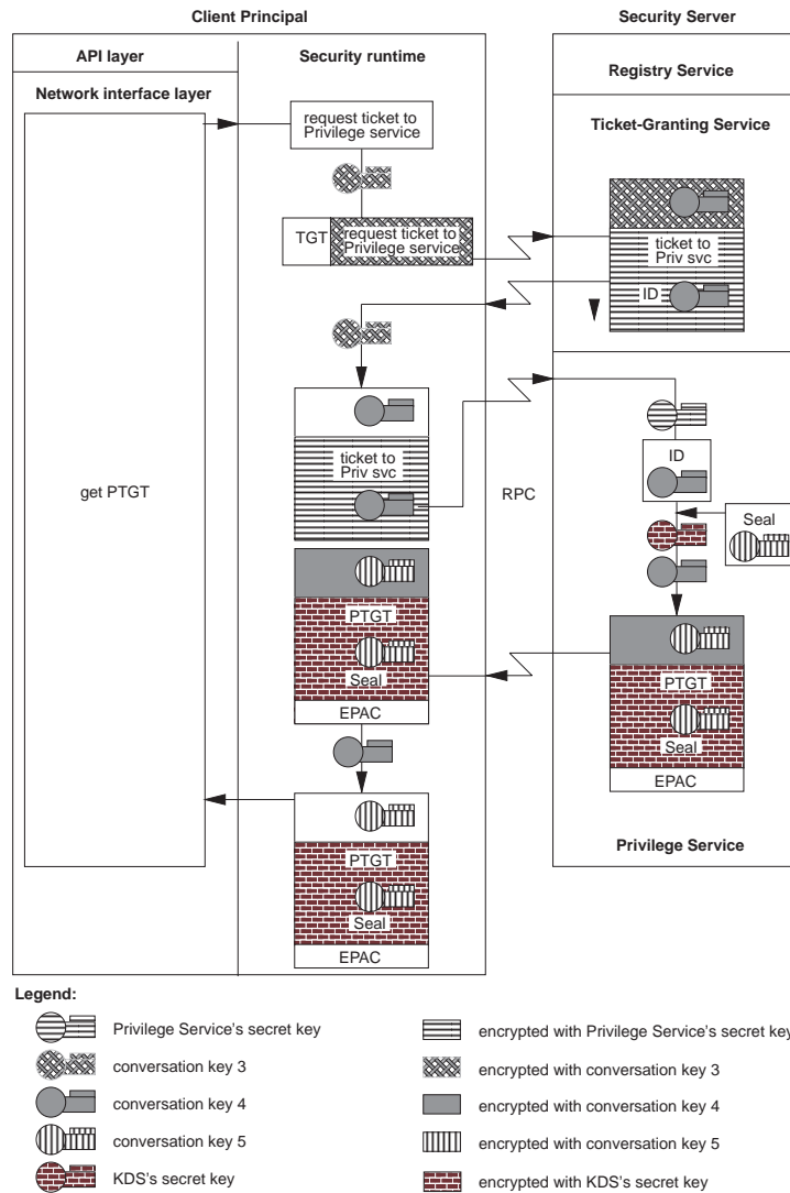
Figure 24–6. Client Acquires PTGT
