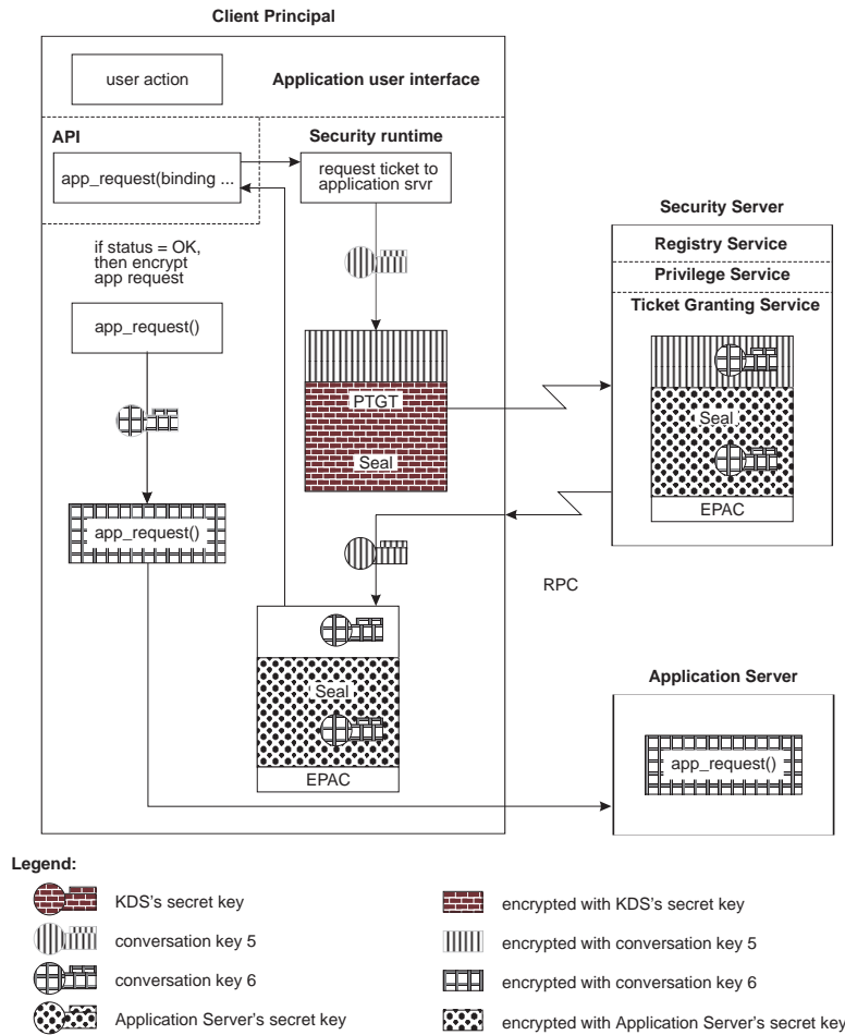
Figure 24–8. Client Principal Makes Application Request
