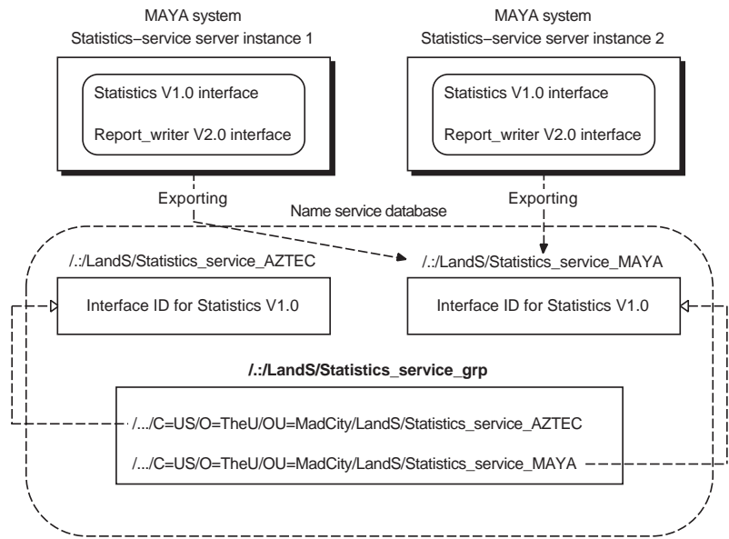
Figure 14–15. Service Model: Interchangeable Instances on One Host
