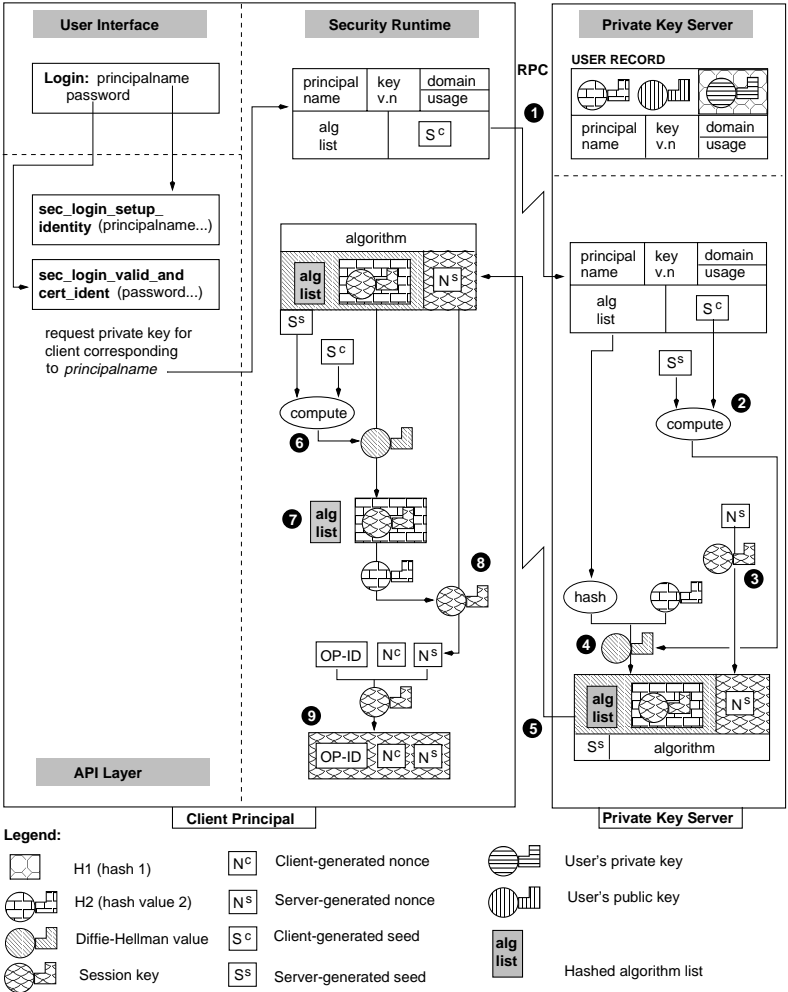
Figure 24–2. Client Initiation of Private Key Acquisition
