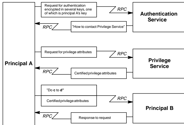
Figure 23–1. Shared-Secret Authentication and DCE Authorization in Brief
