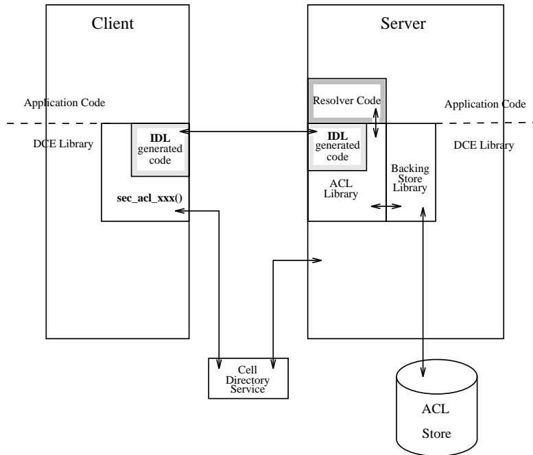
Figure 32–1. ACL Program Interfaces
