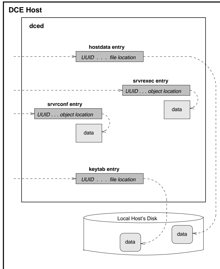
Figure 2–3. Accessing Hostdata
