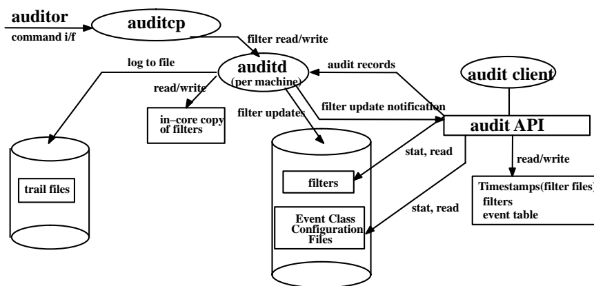
Figure 34–2. Overview of the DCE Audit Service
