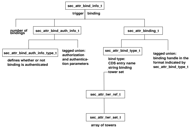
Figure 29–3. The sec_attr_bind_info_t Data Type
