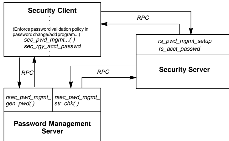
Figure 36–1. Use of Password Management Facility APIs
